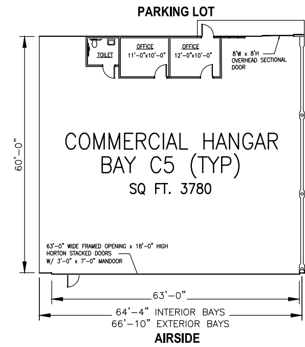
COMMERCIAL HANGAR FLOOR PLAN N.T.S. NORTH
